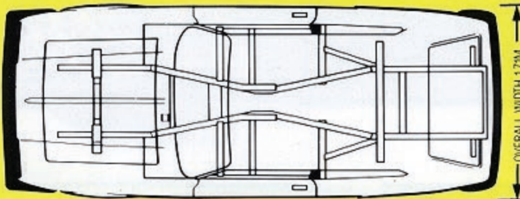
TURNING CIRCLES: BETWEEN KERBS L.40FT., 3IN., R.41FT., 6IN.
